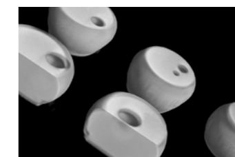
Void in BGA (CT image)
