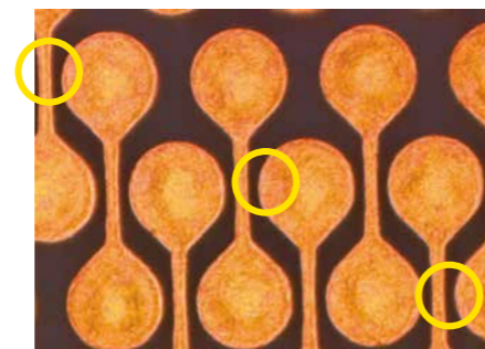
Micro wiring patterns (Type2 head, optical magnification 15x)
