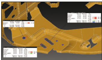
2D hole and slot features
