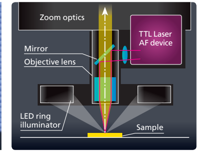
TTL Laser and AF schematic
