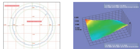
Circle (roundness)
