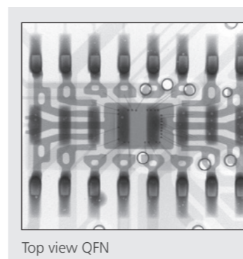
Head-in-Pillow defect
